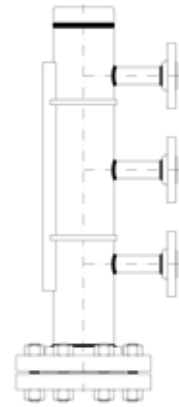
Option 1 with three process connections
