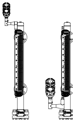
Top/Bottom Mount Offset Configuration
